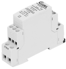
M-Count 2C 2× pulse input (S0)/ M-Bus output
