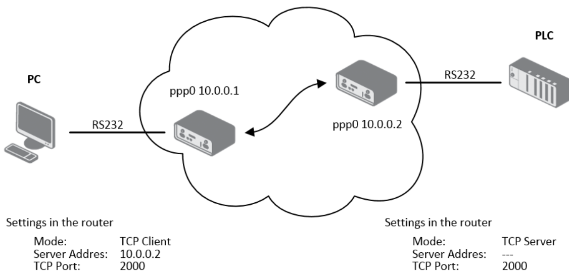
Figure 70: Example of serial interface configuration
