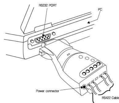
〈 RS422-interface installation example 〉
