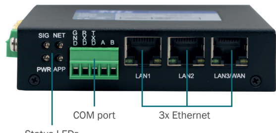
Status LEDs, COM port, 3x Ethernet
