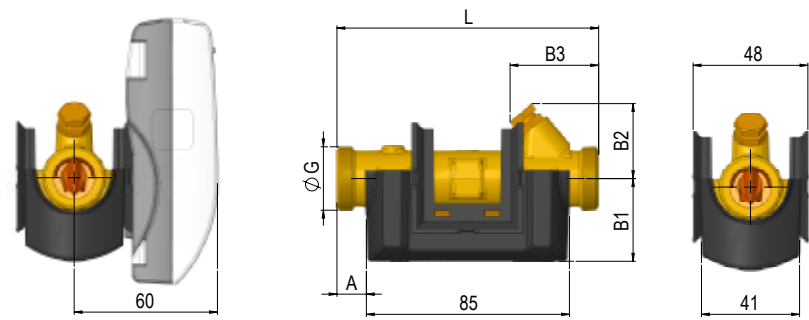
Flow sensor with G¾ and G1 thread connection
