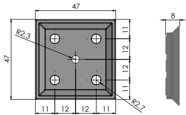
Bracket for wall mounting
