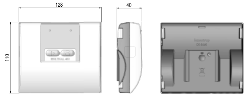
Mechanical measurements for calculator
