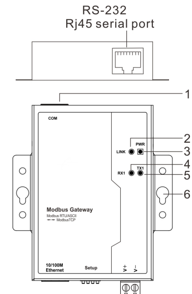
GW1101-1D (RS-232)-P(9~48VDC)
