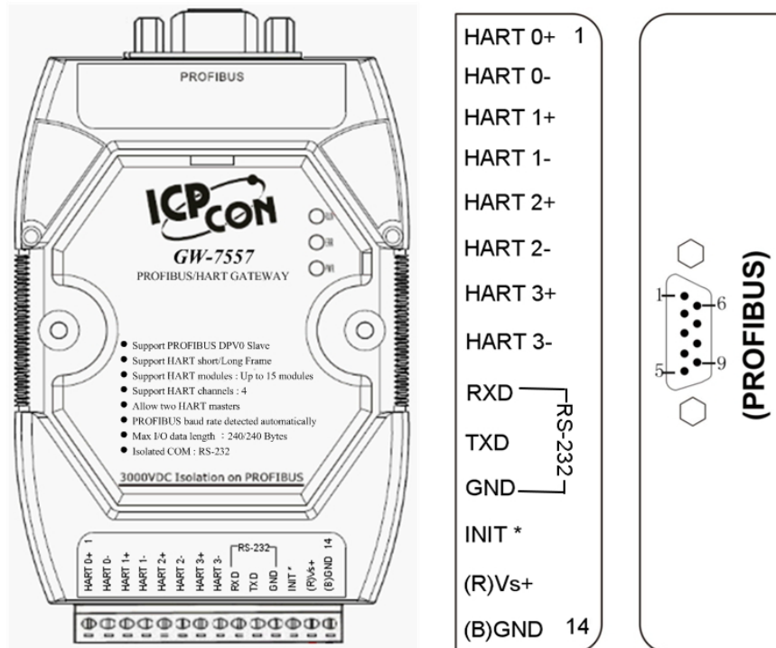
Figure 3 Pin assignment of GW-7557
