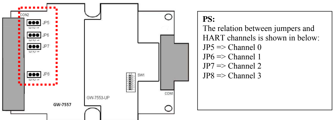
Figure 14 Jumpers of GW-7557
