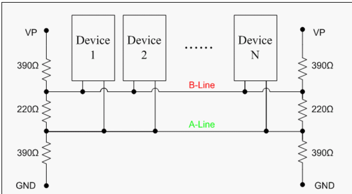
Figure 5 PROFIBUS connection
