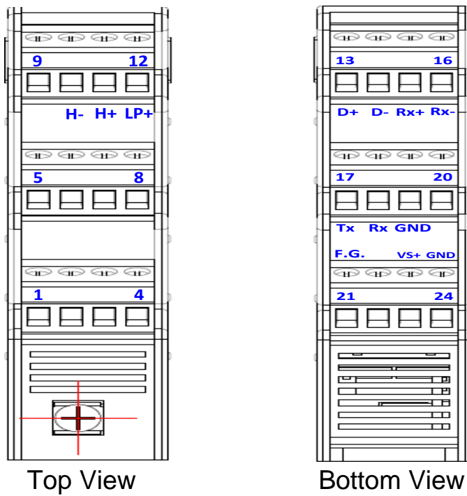
Figure 3.2: Pin assignment of HRT-310
